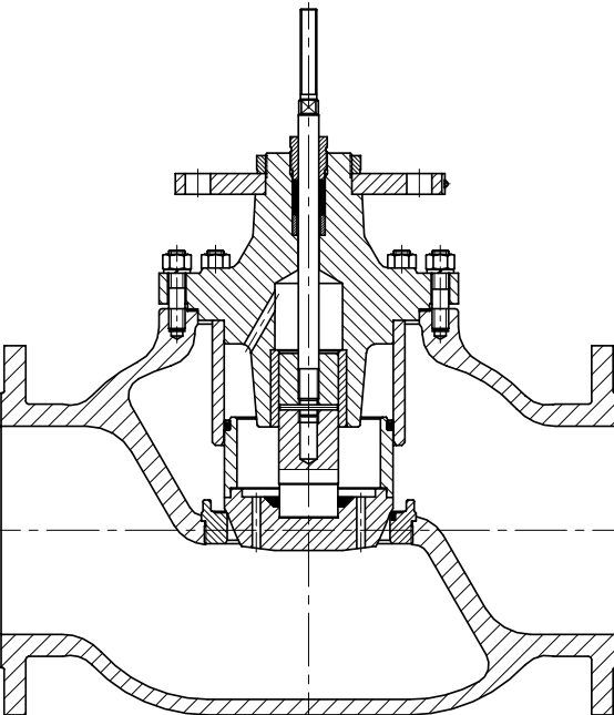
b) with balanced plug
