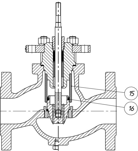
b) with balanced plug
