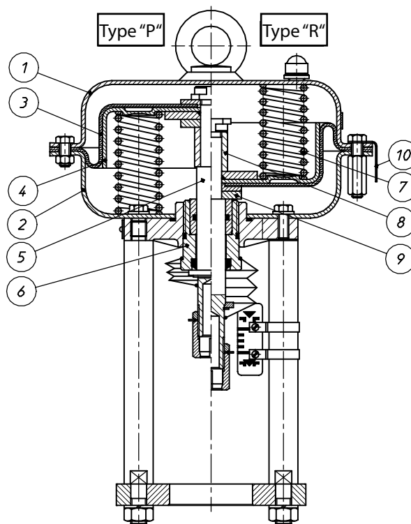
Fig. 5. P/R multispring pneumatic actuator
