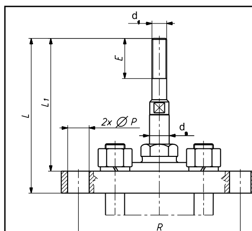
Fig. 6. Valve connection dimensions
