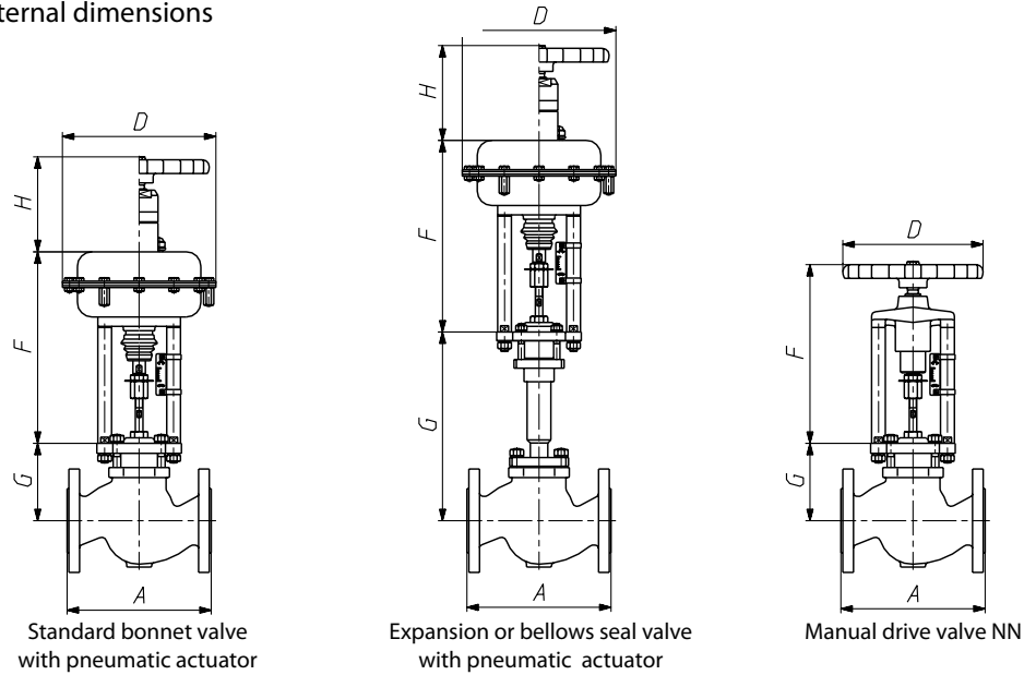
Fig. 7. Valve external dimensions
