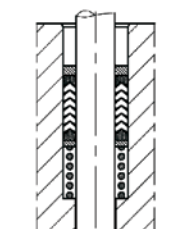
Packing (PTFE-V)
