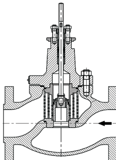
Figr. 1b. Valve BR 12B - balanced plug
