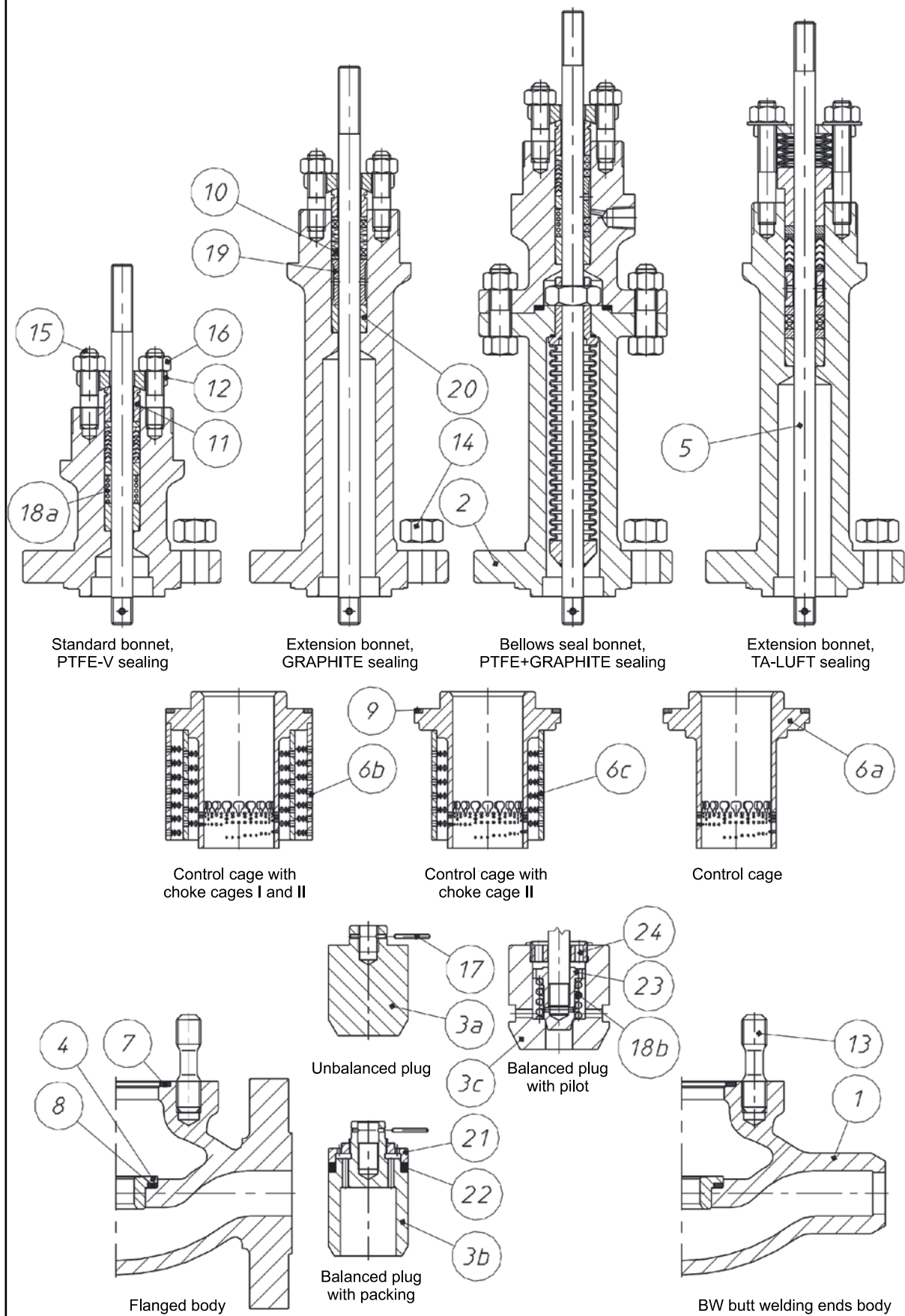
Fig. 1d. Control valve
