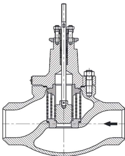
Figr. 1a. Valve BR 12B - unbalanced plug
