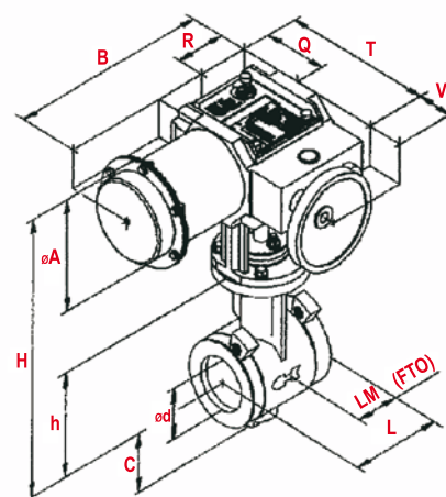
Flangeless valve - Sandwich Actuator P/R 99-1
