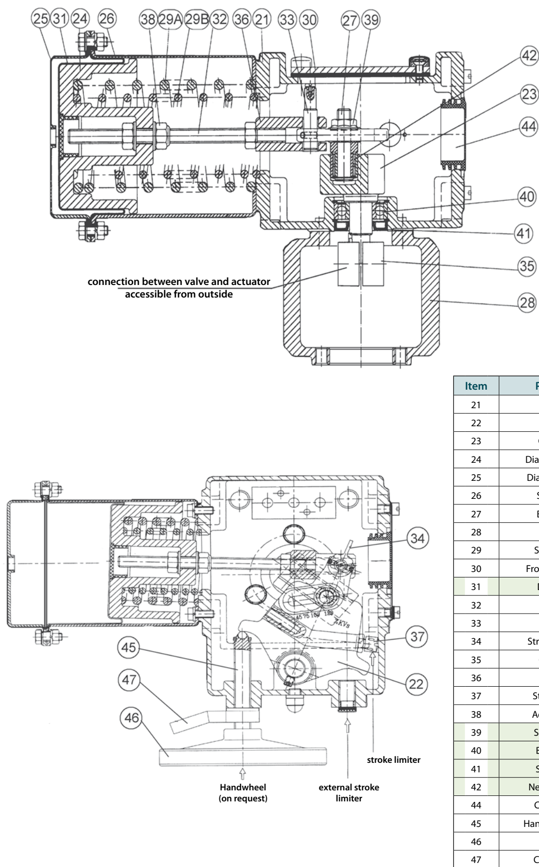
Fig. 2 Rotary pneumatic actuator (spring and diaphragm) type P/R-99
