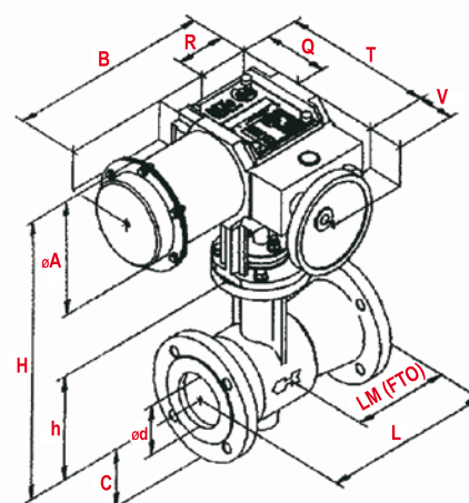
Flanged valve Actuator P/R 99-1
