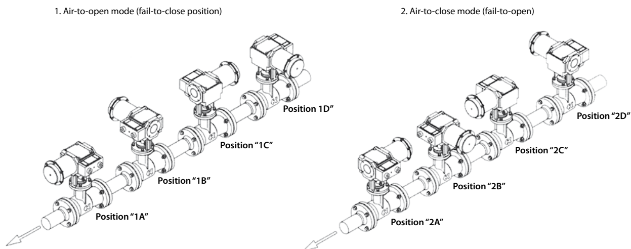
Fig. 5 Possible actuator type P/R-99 positions to valve axis.
